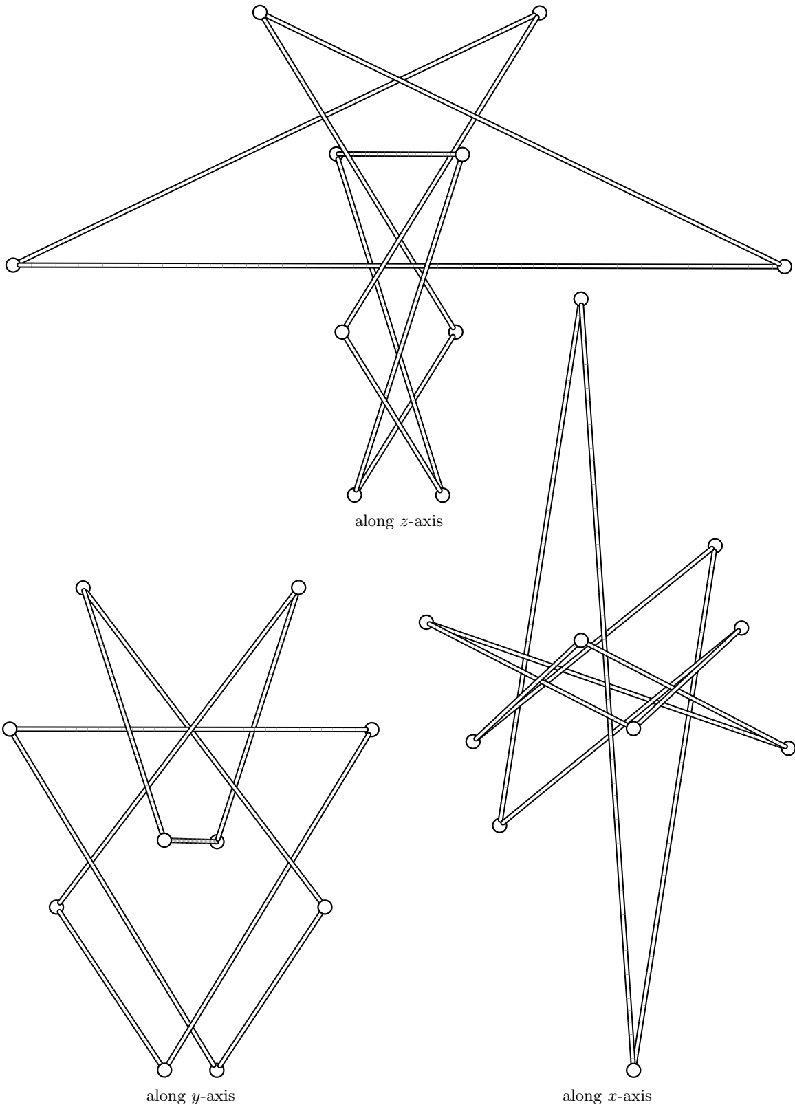
Minimal-stick candidate for 10_{124} viewed along its three principal axes.
