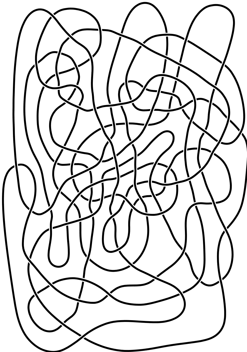
111-crossing unknot from paper by Lewin, Gan & Bruckstein
